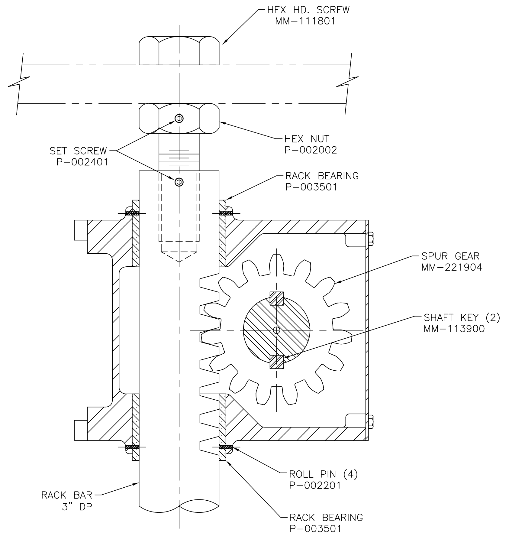
SECTION B-B
